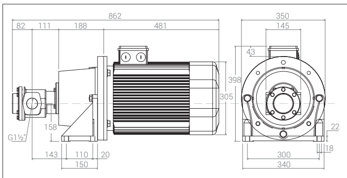
FOM 570- FOM 590 ( 15 kW ) weight: 158 kg
