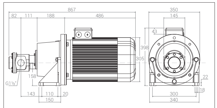
FOM 570- FOM 590 ( 18,5 kW ) weight: 184 kg
