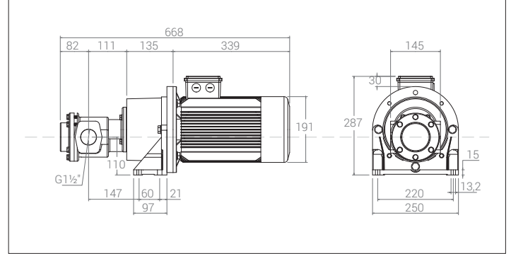
FOM 570- FOM 590 ( 3,0 kW ) weight: 47 kg
