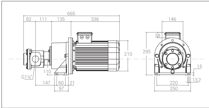
FOM 570- FOM 590 ( 4,0 kW ) weight: 53 kg
