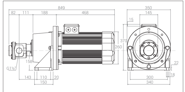
FOM 570- FOM 590 ( 11 kW ) weight: 109 kg
