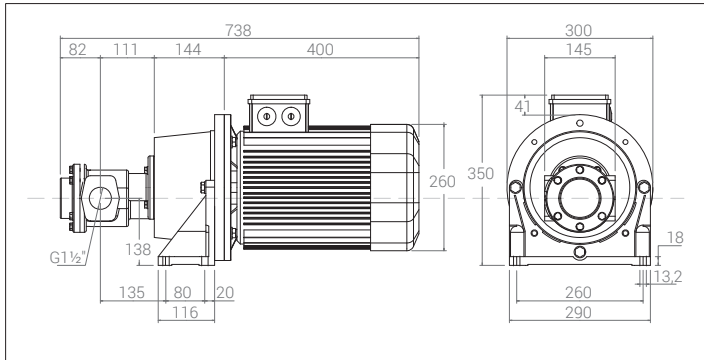
FOM 570- FOM 590 ( 7,5 kW ) weight: 106 kg
