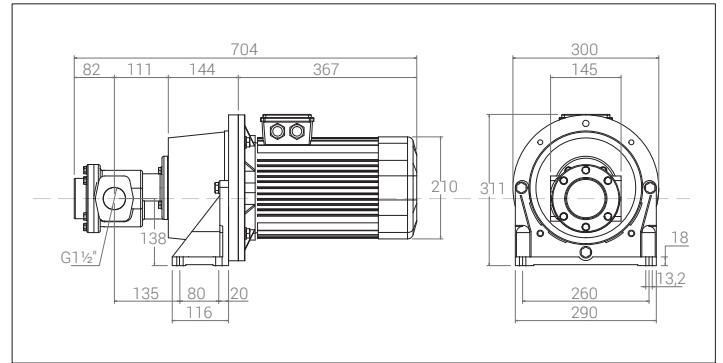
FOM 570- FOM 590 ( 5,5 kW ) weight: 70 kg
